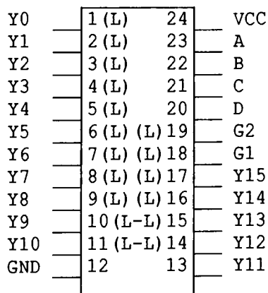
74LS154 4:16 Decoder/Demultiplexer
