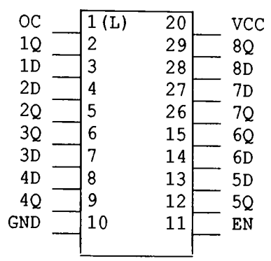
74LS373 Octal Latch
