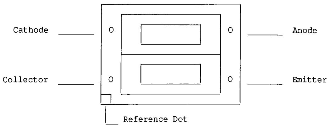
FPA104 Infrared Phototransistor
