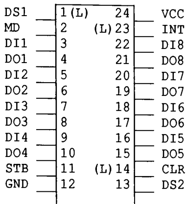
8212 8-Bit Input/Output Port
