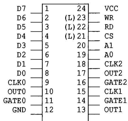
8254 Programmable Timer
