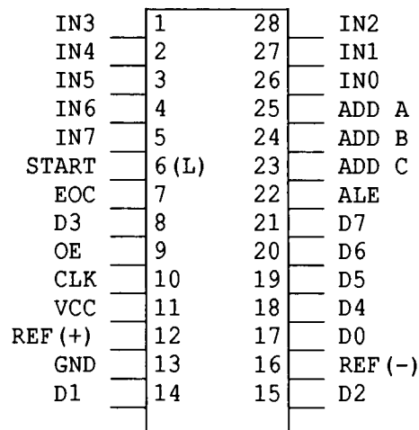
ADC0808 8-Bit 8-Channel A/D Converter
