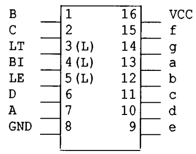
4511 Binary to BCD Latch/Decoder Driver
