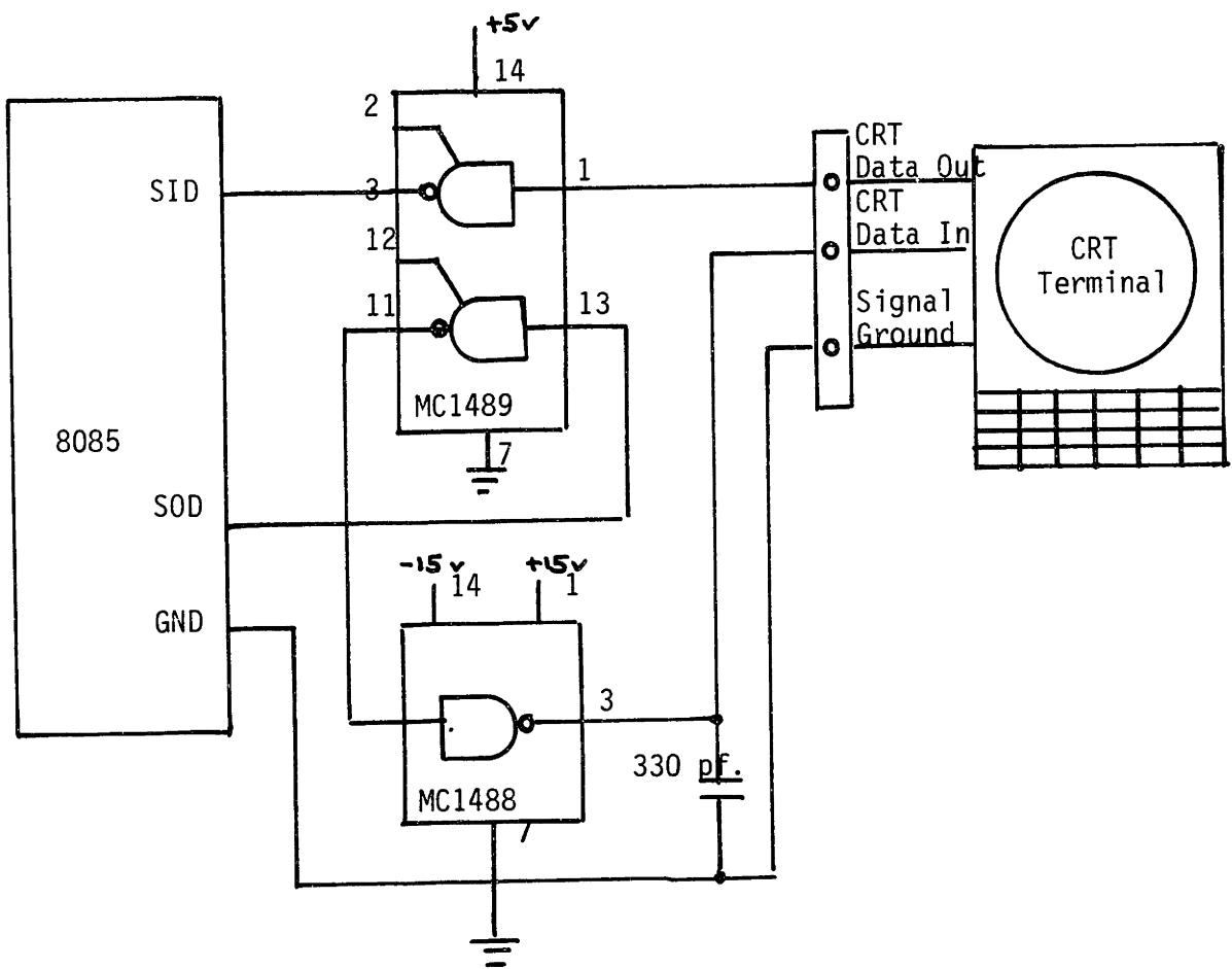
Figure 13. RS-32C Interface Circuit
